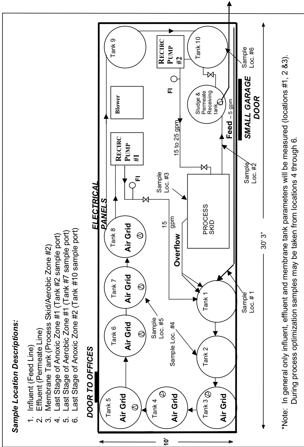
Figure 3-2 Twelve Pines STP MBR Demonstration Layout (April 10 – August 26, 2001)
