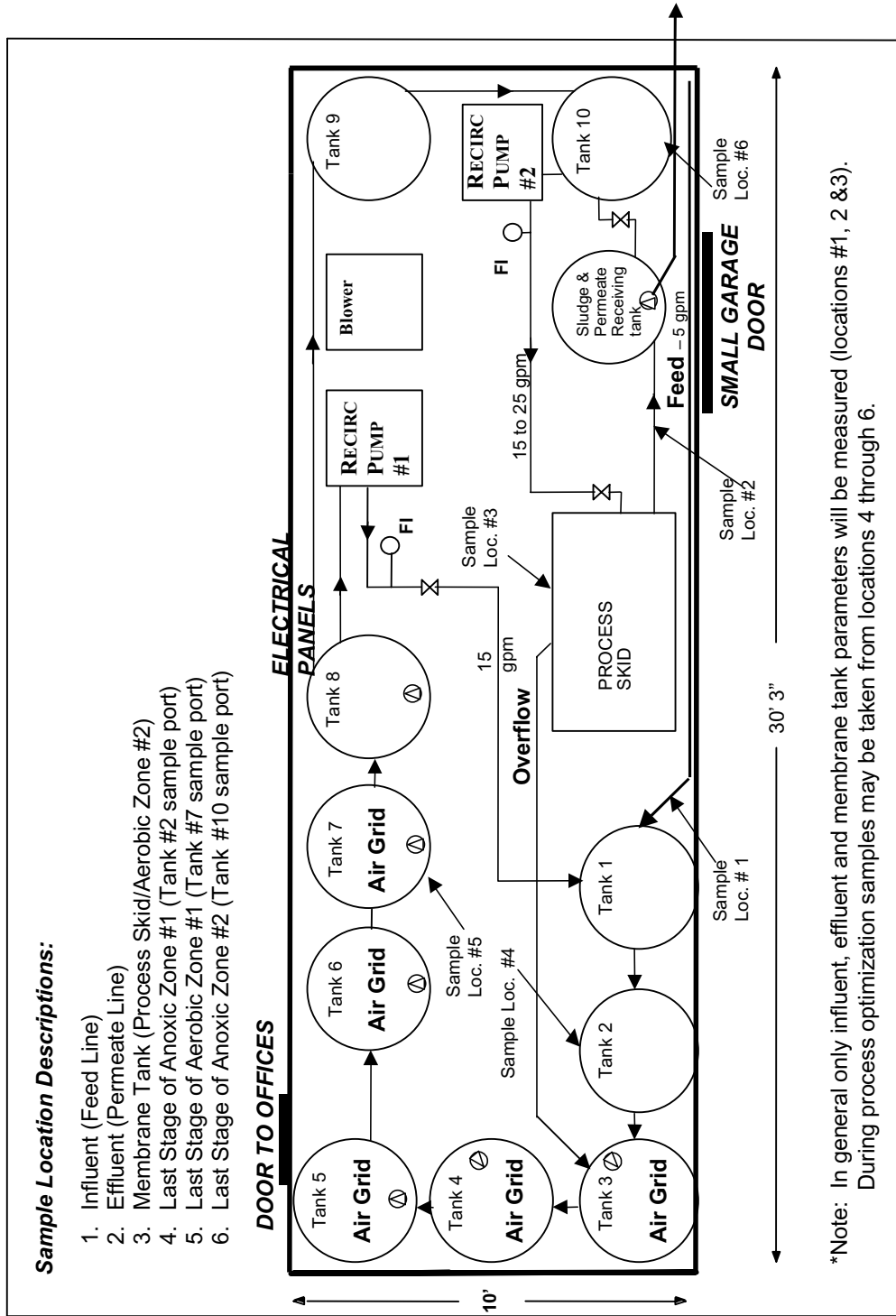
Figure 3-6 Twelve Pines STP MBR Demonstration Layout (November 7, 2001 – February 7, 2002)
