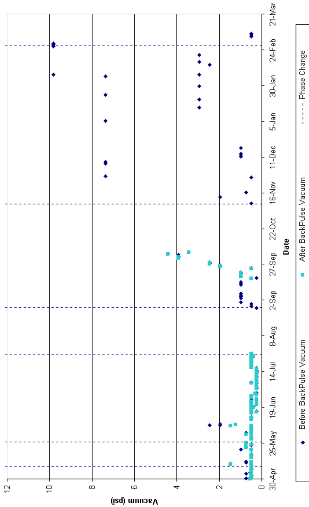
Figure 4-2: Before and after backpulse vacuum.
