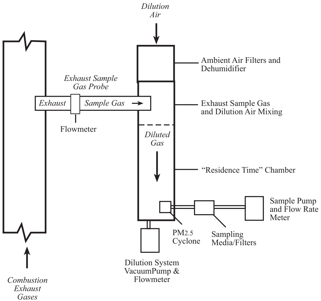
Figure 2. Dilution sampling system schematic
